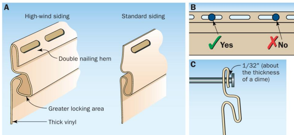
Figure 5. Fastening for high-wind vinyl siding
