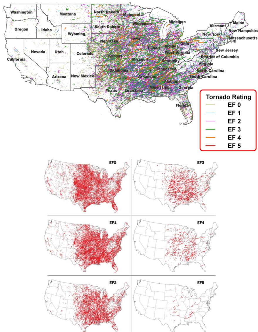
Figure 2. Reported tornadoes in the contiguous United States by EF intensity, from 1950 through 2021. (Data source: NOAA/NWS Storm Prediction Center)
